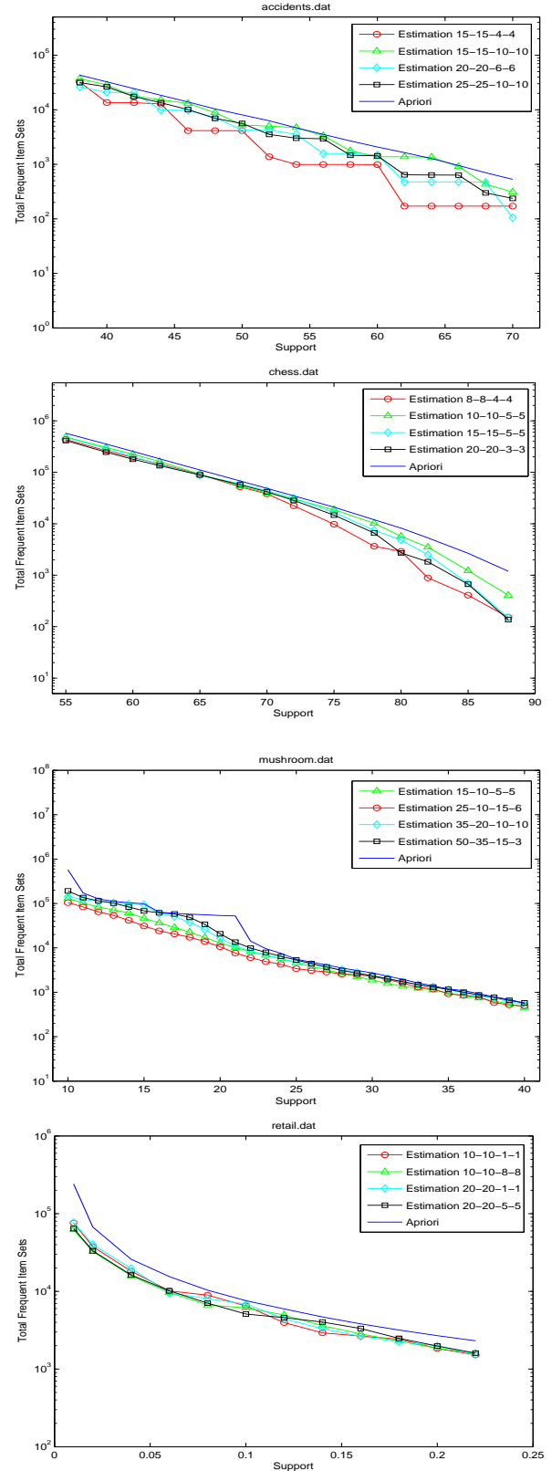
Figure 6: Estimation of Total Number of Frequent Itemsets
