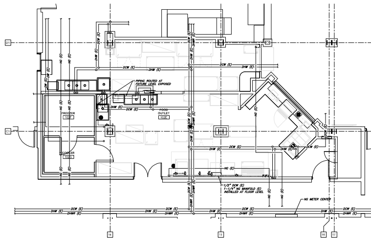
PLUMBING PLAN (EXISTING CONDITIONS - WATER AND GAS) SCALE: 1/4" = 1'-0"
