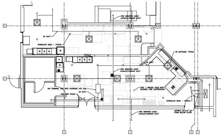
MECHANICAL PLAN (EXISTING CONDITIONS) SCALE: 1/4" = 1'-0"
